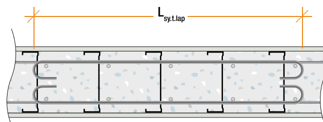
Fig D26: 14.6.7(D) Horizontal Wall Bar Lap Detail
